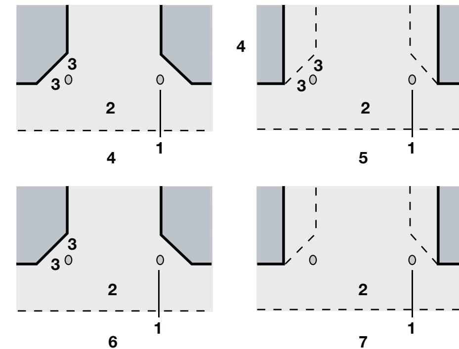
1. Bollards 2. Footway 3. 1.5 pedestrian/vehicle visibility dispaly 4. Splays cut out of buildings or walls 5. Entrance widened by 1.5m on each side 6. Buildings or walls set back 1.5m behind back edge of footway 7. Buildings set back and entrance widened by less than 1.5m each
