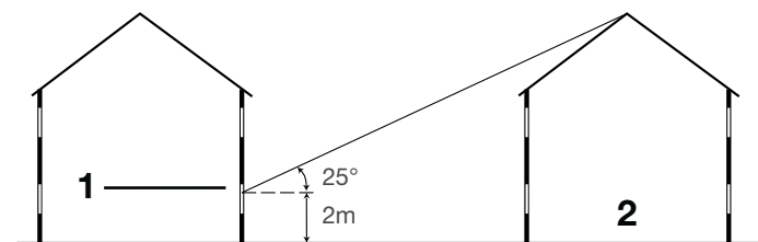
1. Reference line for daylight calculation 2. Obstructing building
